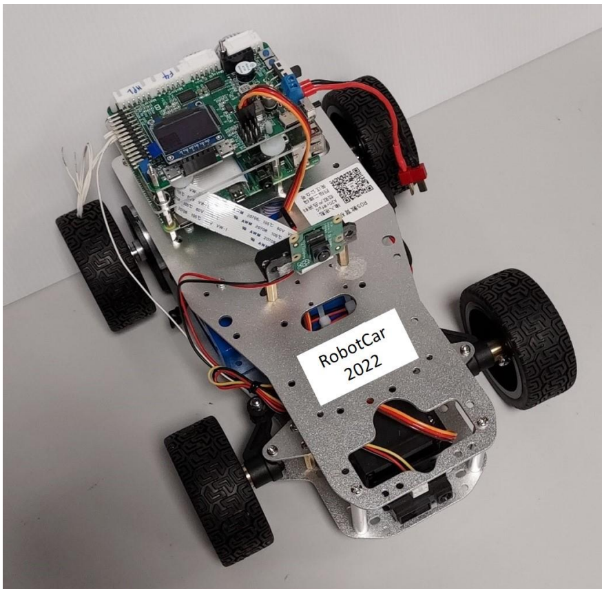
Fig 8 – Full Top view with Picamera and IR sensor
