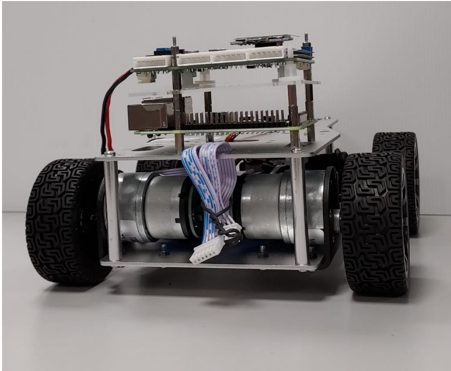
Fig 7 – Full Back view
