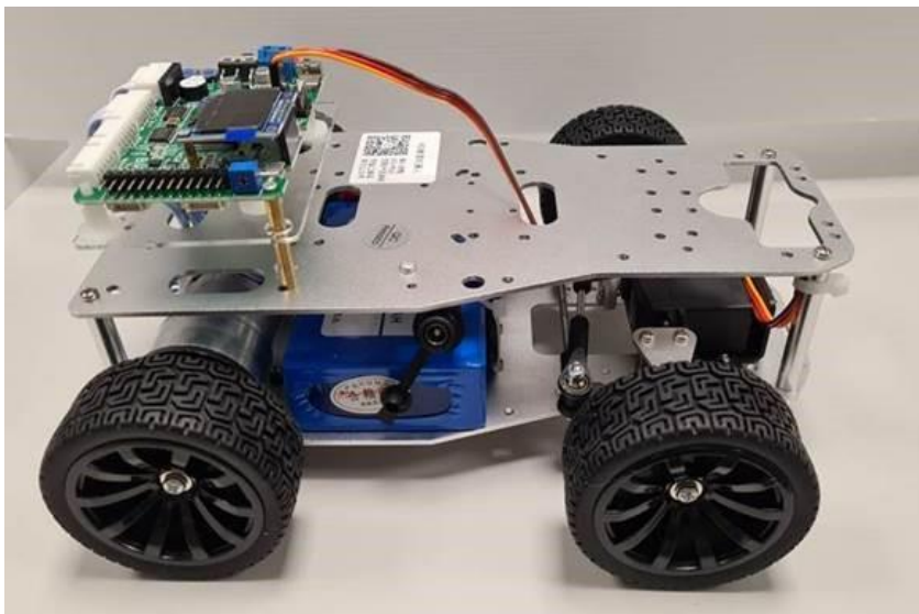
Fig 1b – Supplier's version (M2.5 pillars – please replace by M2 pillars, see Fig 2 onwards)
